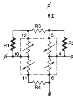
Figure 5 - Offset TC
