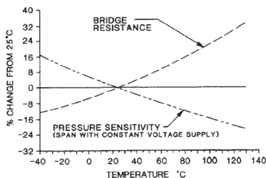
Figure 3 - Temperature Dependence of Bridge Resistance and Pressure Sensitivity
