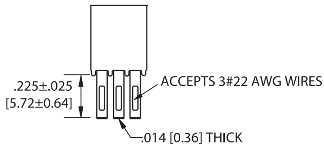
EYELET (P)
