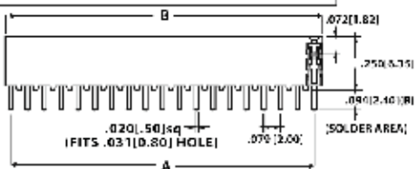
QUAD READOUT, STRAIGHT TAIL SHOWN
