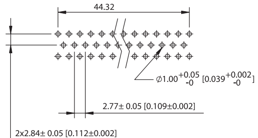
50 Positions Machined Pin (W/O Rear Cover)
