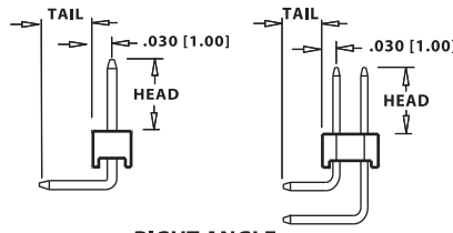
RIGHT ANGLE
