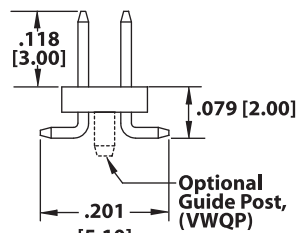
(VWQS), Without Guide Post (VWQP), With Guide Post
