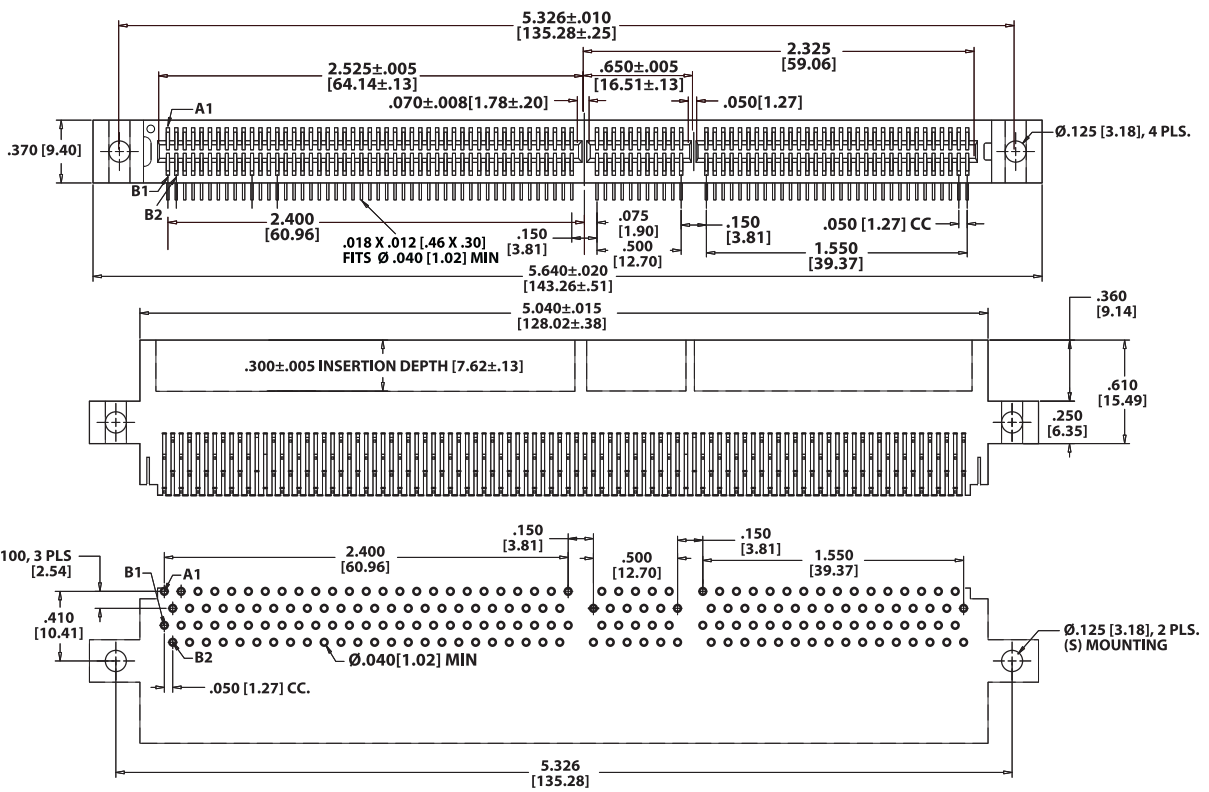
BOARD LAYOUT, CONNECTOR SIDE G B B 92 D H A S - S250, 64 BIT, 5 VOLT
