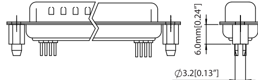
h : 3 Rivet+2 Prong Boardlock \phi 3.2 \times 6.0 \text{ L} [0.13 x 0.24]
