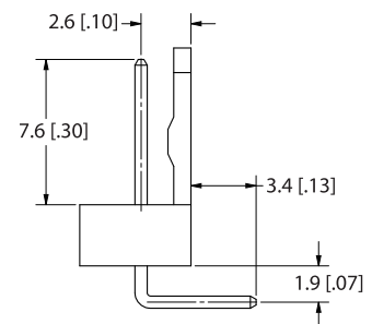
SWR25X-NRTC-S__-RB-BA (TYPE 1)
