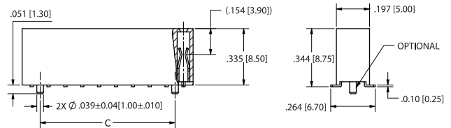
SFM850 Series Dual Row
