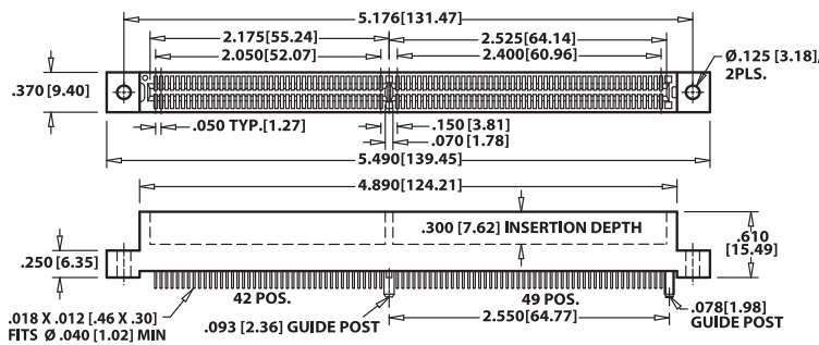
GBB91DHHDD-S578, 91 (42/49) POSITIONS
