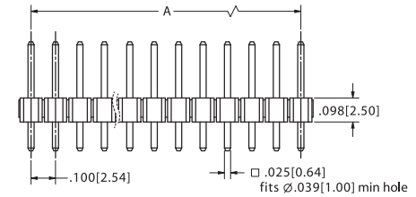
SINGLE READOUT, STRAIGHT TAIL SHOWN
