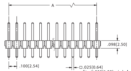
DUAL READOUT, STRAIGHT TAIL SHOWN
