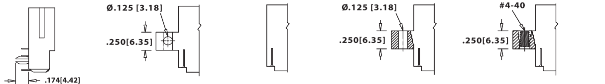
BOARD LOCK (R) (with no mounting ears) SIDE MOUNTING (S) NO MOUNTING EARS (N) FLUSH MOUNTING (D) THREADED INSERT (T)
