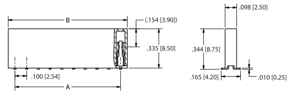
SFM850 Series Dual Row
