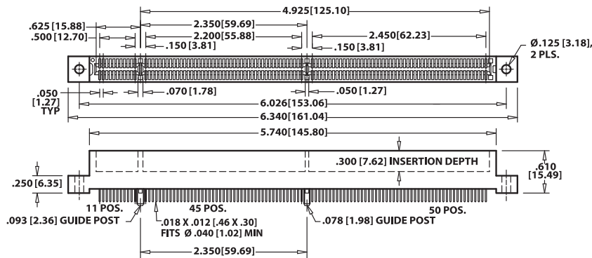
GBB106DHHDD-S578, 106 (11/45/50) POSITIONS
