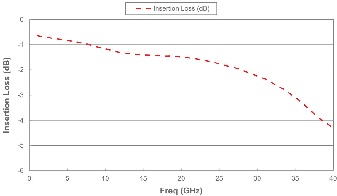
Figure 10. Insertion Loss of PE42524 on 8 mil Rogers 4003 PRT44405 Substrate Carrier
