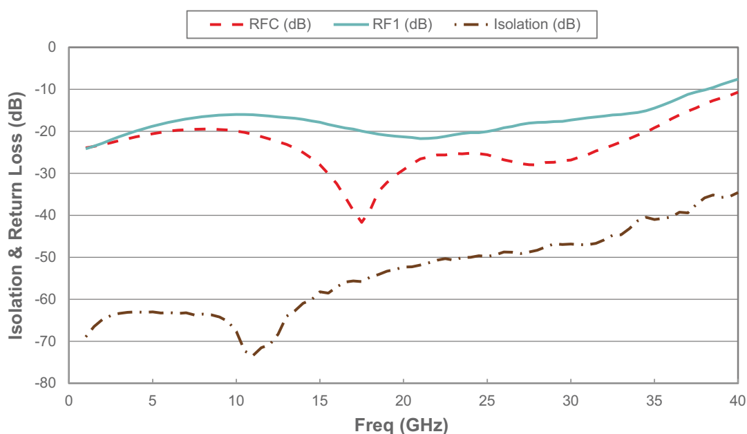
Figure 9. Isolation and Return Loss of PE42524 on 10 mil Alumina Substrate Carrier
