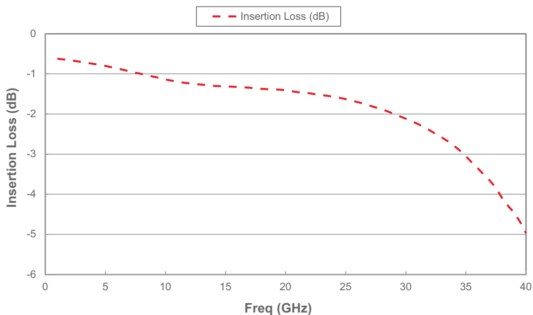
Figure 8. Insertion Loss of PE42524 on 10 mil Alumina Substrate Carrier
