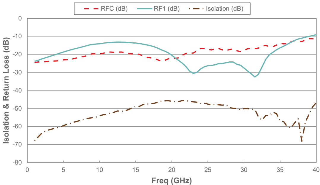
Figure 11. Isolation and Return Loss of PE42524 on 8 mil Rogers 4003 PRT44405 Substrate Carrier
