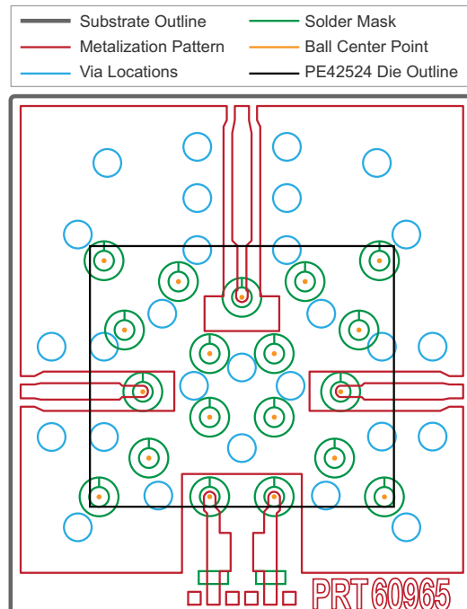
Figure 2b. PRT60965 10 mil Alumina Substrate Metallization and Via Pattern Recommended for Maximum Isolation
