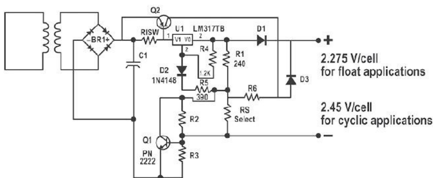
Dual stage current limited SLA battery charger
