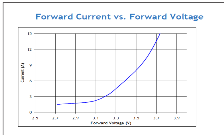
Figure 3: Typical I-V curve of a Big Chip LED
