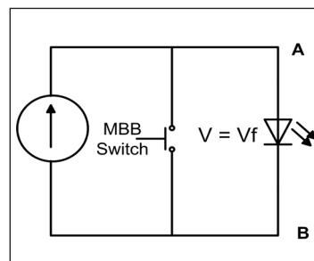
Figure 4b: MBB switch open
