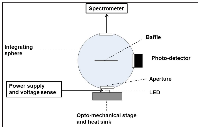
Figure 1: Schematic of Test Station
