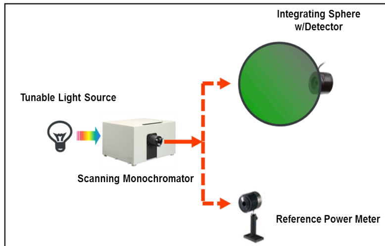
Figure 2: Substitution method of calibration
