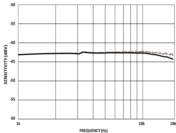
Figure 3. Microphone Response with Added Washer and No Seal (Dotted Lines)
