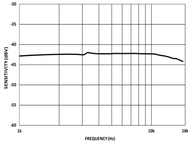
Figure 2. Baseline Response of a Bottom Port MEMS Microphone
