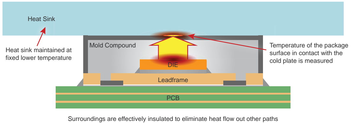
Figure 1 • Example of \Theta_{JC} Measurement (*)
