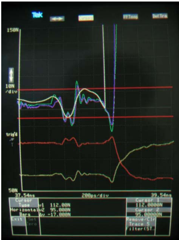
Figure 9c: TDR at D0 of Port B
