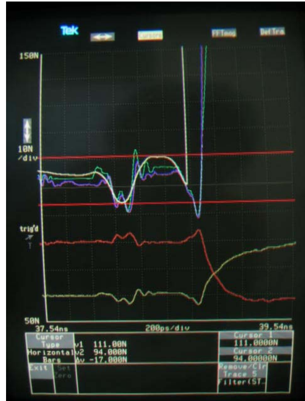
Figure 8b: TDR at D1 of Port A
