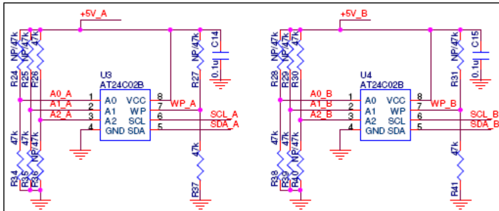
Figure 6: Schematic of EEPROM
