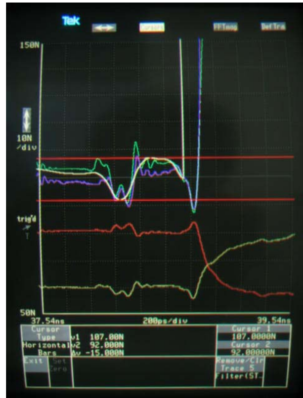
Figure 9d: TDR at CLK of Port B
