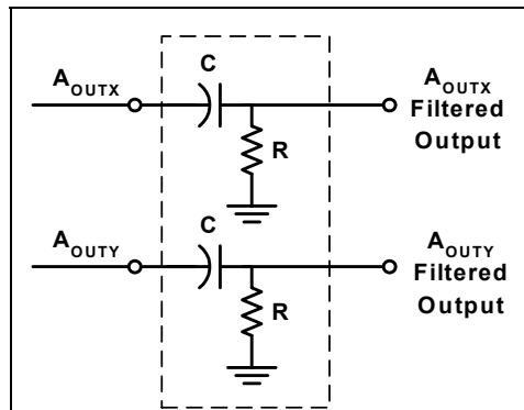
Figure 7: High Pass Filter
