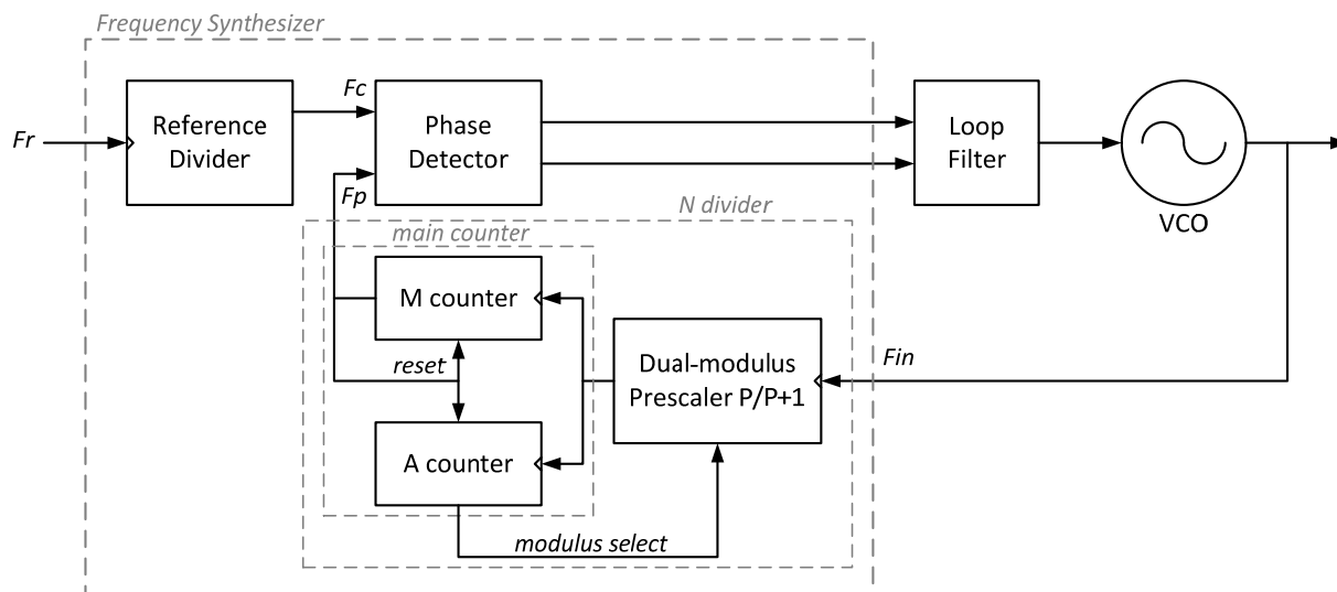
Figure 1. PLL Integer-N PLL Functional Block Diagram with a Dual Modulus Prescaler
