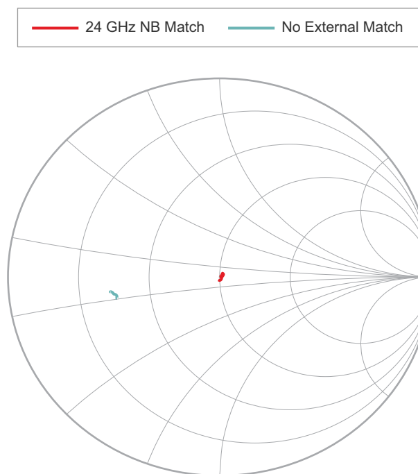
Figure 10. Smith Chart Representation of the Narrowband Match Port Impedances
