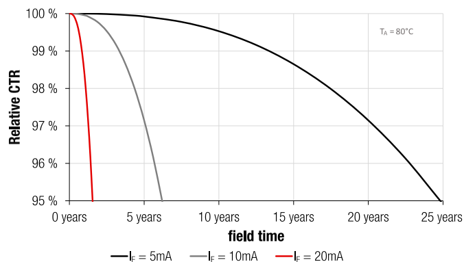
Figure 3: Forward current dependency on expected average CTR degradation with field time. Parameters for field use: 100% duty cycle, 80°C ambient temperature, forward currents as indicated in the graph. Stress test parameters: 1000 h test, 110°C test temperature, 30 mA forward current.
