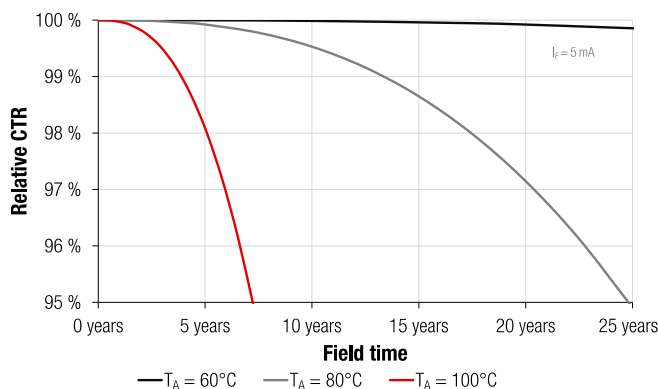
Figure 4: Temperature dependency on expected average CTR degradation with field time. Parameters for field use: 100% duty cycle, 5 mA forward current, ambient temperatures as indicated in the graph. Stress test parameters: 1000 h test, 110°C test temperature, 30 mA forward current.
