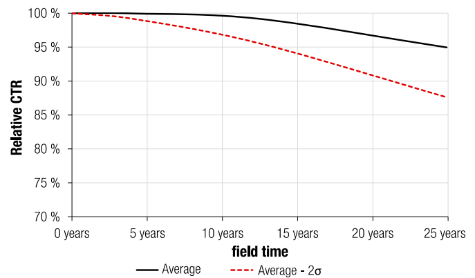
Figure 2: Expected CTR degradation with field time. Parameters for field use: 100% duty cycle, 80°C ambient temperature, 5 mA forward current. Stress test parameters: 1000 h test, 110°C test temperature, 30 mA forward current
