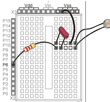
Figure D-7 Resistor, Photoresistor, and Capacitor Wiring Diagram
