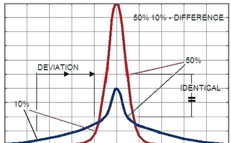
Figure 2: FWHM value does not give unambiguous information of an optical component. These two lenses have the same FWHM value, but they perform in a very different way.
