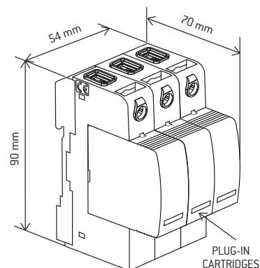
3 Poles
