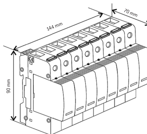
8 Poles
