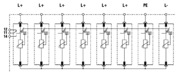
8 Poles
