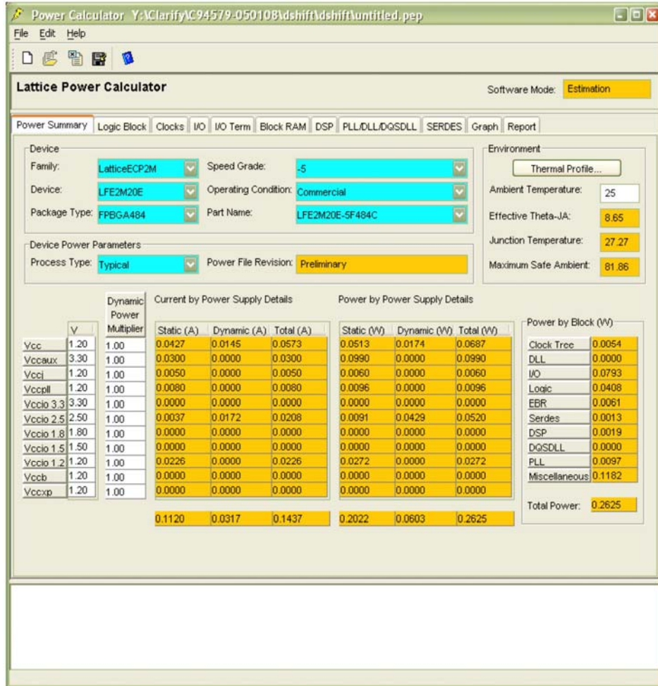
Figure 1 - The Power Calculator can be used at any point in the design cycle. Early estimates of toggle rates can later be replaced with simulation results. The Power Calculator accurately calculates current and power for all architectural elements and provides a thermal profile to model real system conditions
