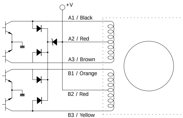
UNI-POLAR DRIVE
