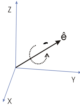
Figure 4. Euler axis and angle.
