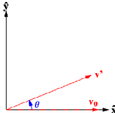
Figure 3. 2D rotation example.
